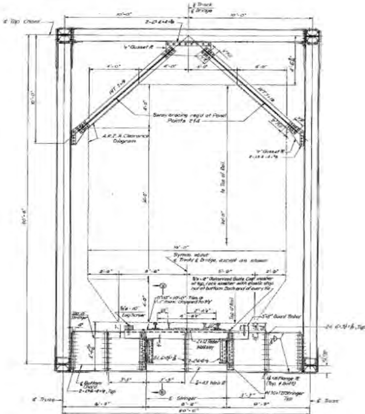
SECTION AT INTERIOR FLOORBEAM BASCULE BRIDGE OVER THREE MILE CREEK
